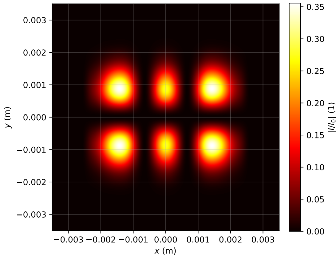
Intensity profile I(x, y, z = 3.025)/I_0 , P_{in}=1.0P_{cr} , artificial time
